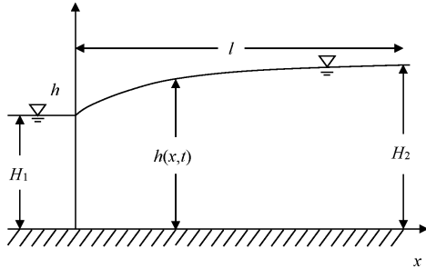
Fig. 2 Schematic diagram of groundwater table profile
